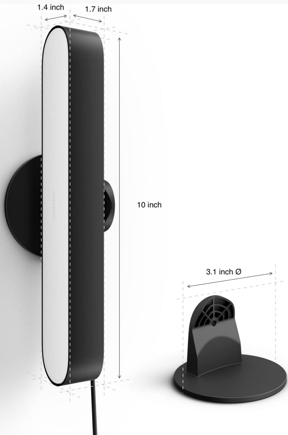
Figure 6: Dimensions of the Philips Hue Play Light Bar.
