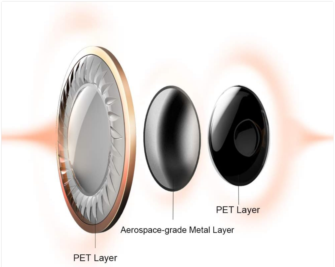
Image 3.1: Internal structure of the earbud, illustrating the triple driver configuration.
