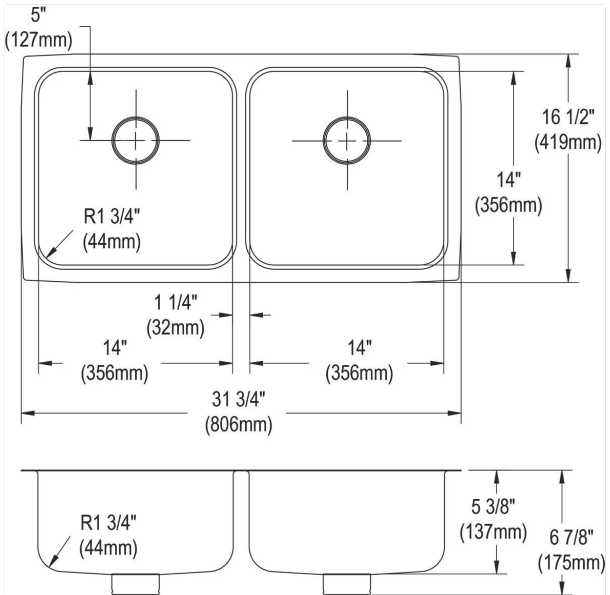
Figure 1: Detailed dimensions and specifications for the Elkay ELUHAD321655PD sink, showing overall size, bowl dimensions, and drain placement.
