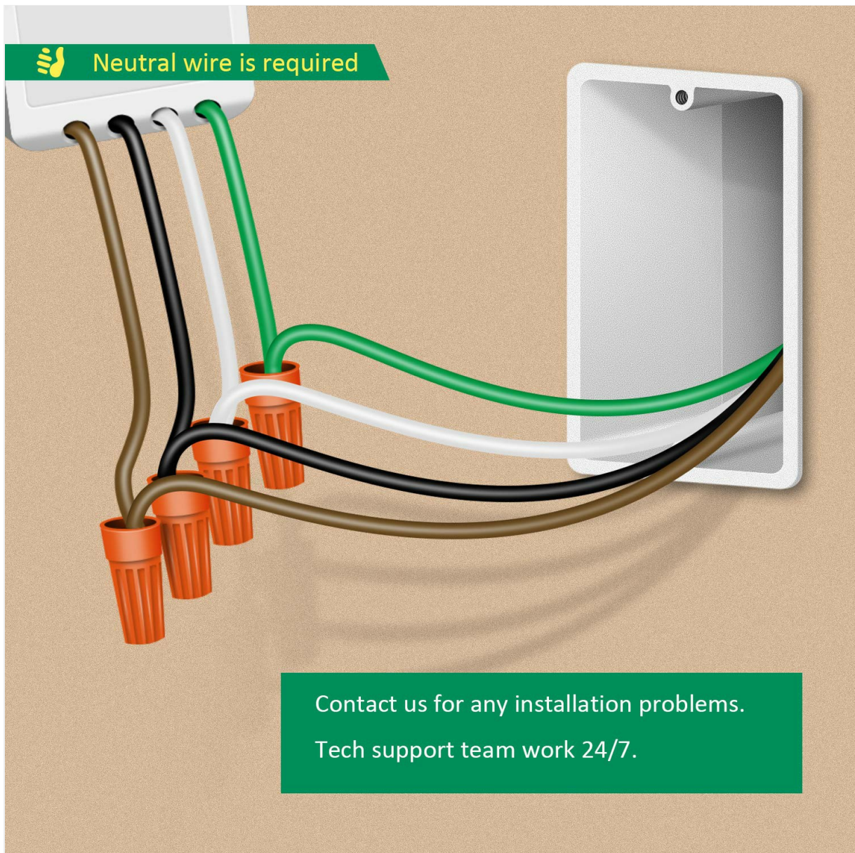
Figure 4.1: Diagram showing the required neutral wire connection for the smart switch installation.
