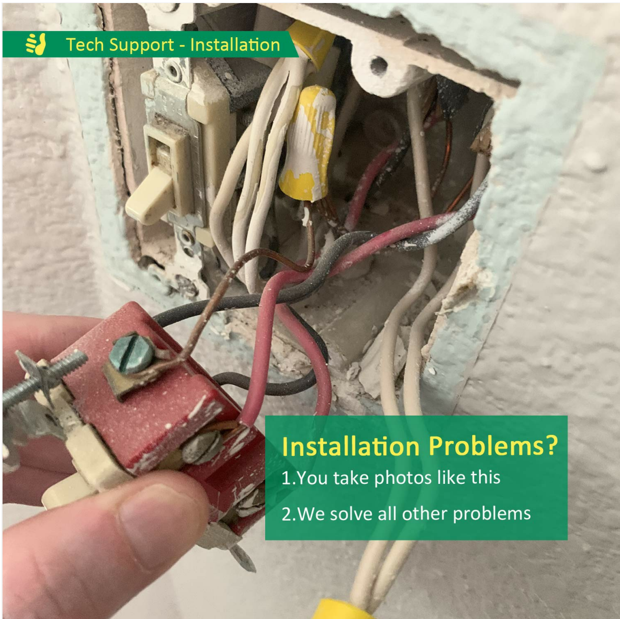
Figure 4.2: Example of existing wiring in a wall box. For installation problems, taking photos like this can help our tech support team.
