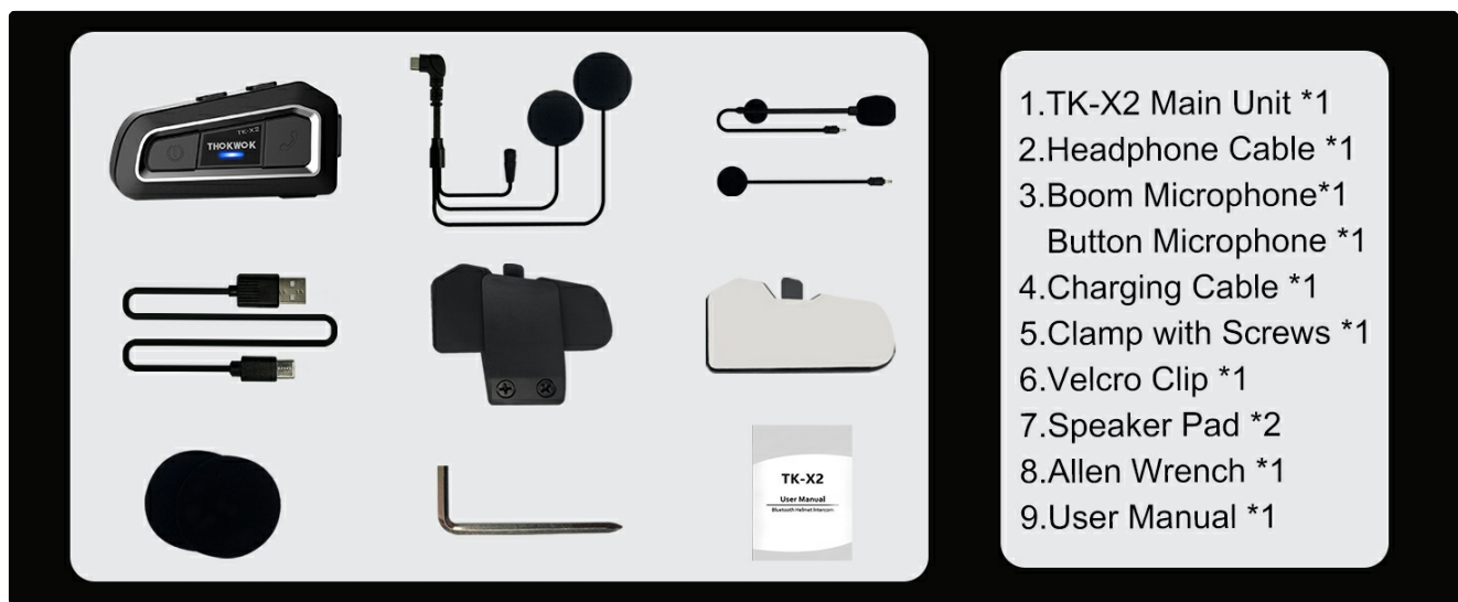
Figure 1: All components included in the THOKWOK TK-X2 package.
