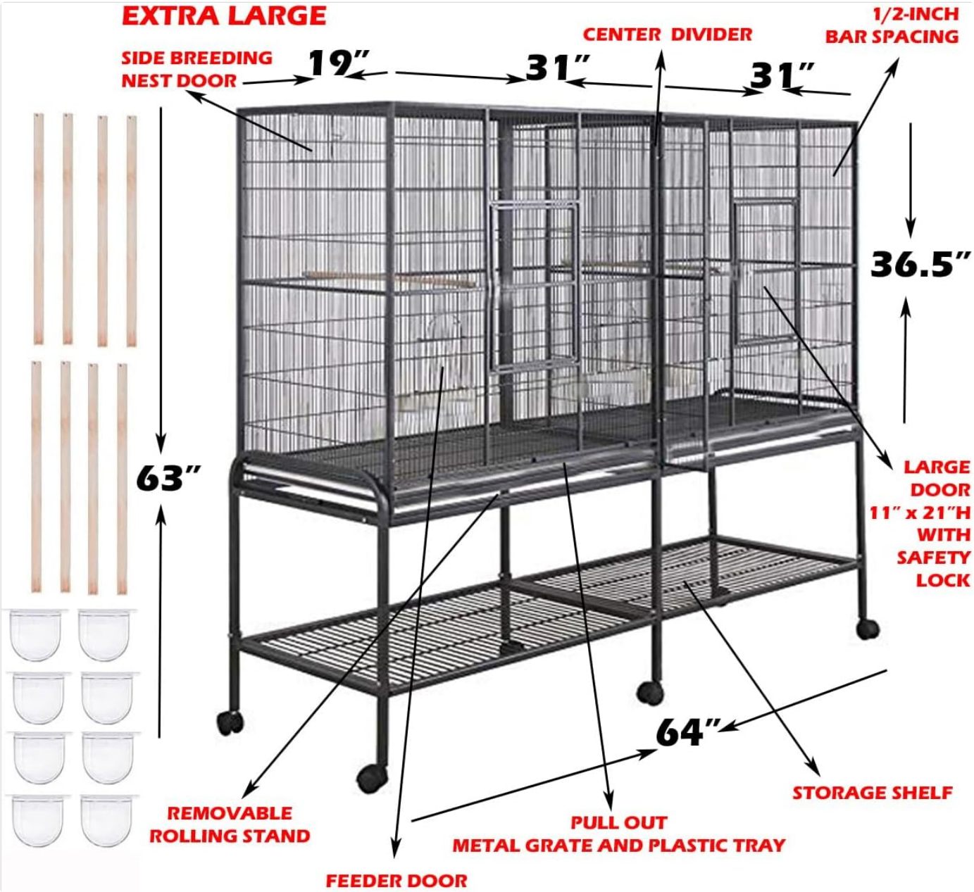
Figure 1: Overview of all cage components and key dimensions.
