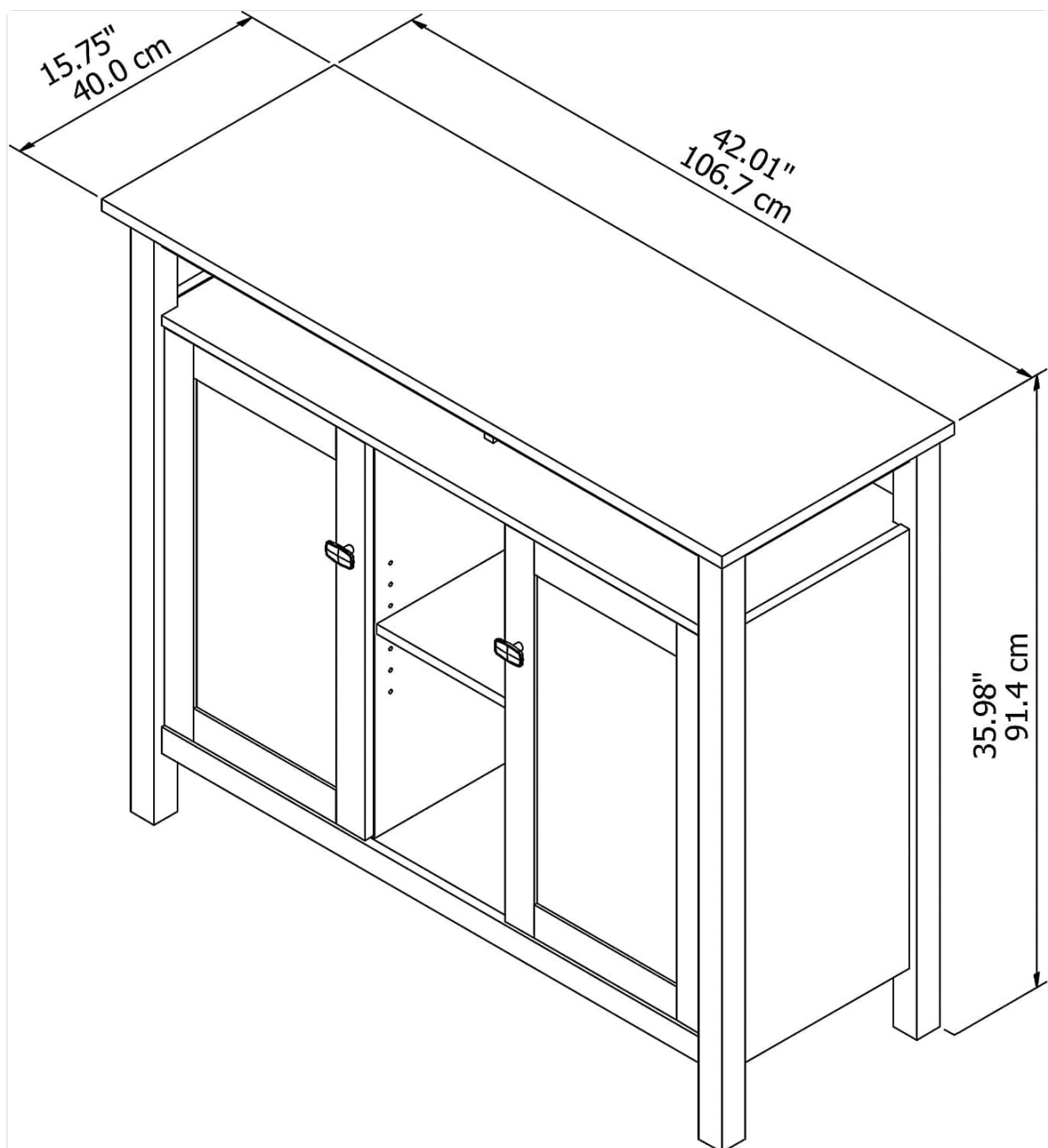
Image 8.1: Dimensional diagram of the console table, indicating depth (15.75"), width (42.01"), and height (35.98").
