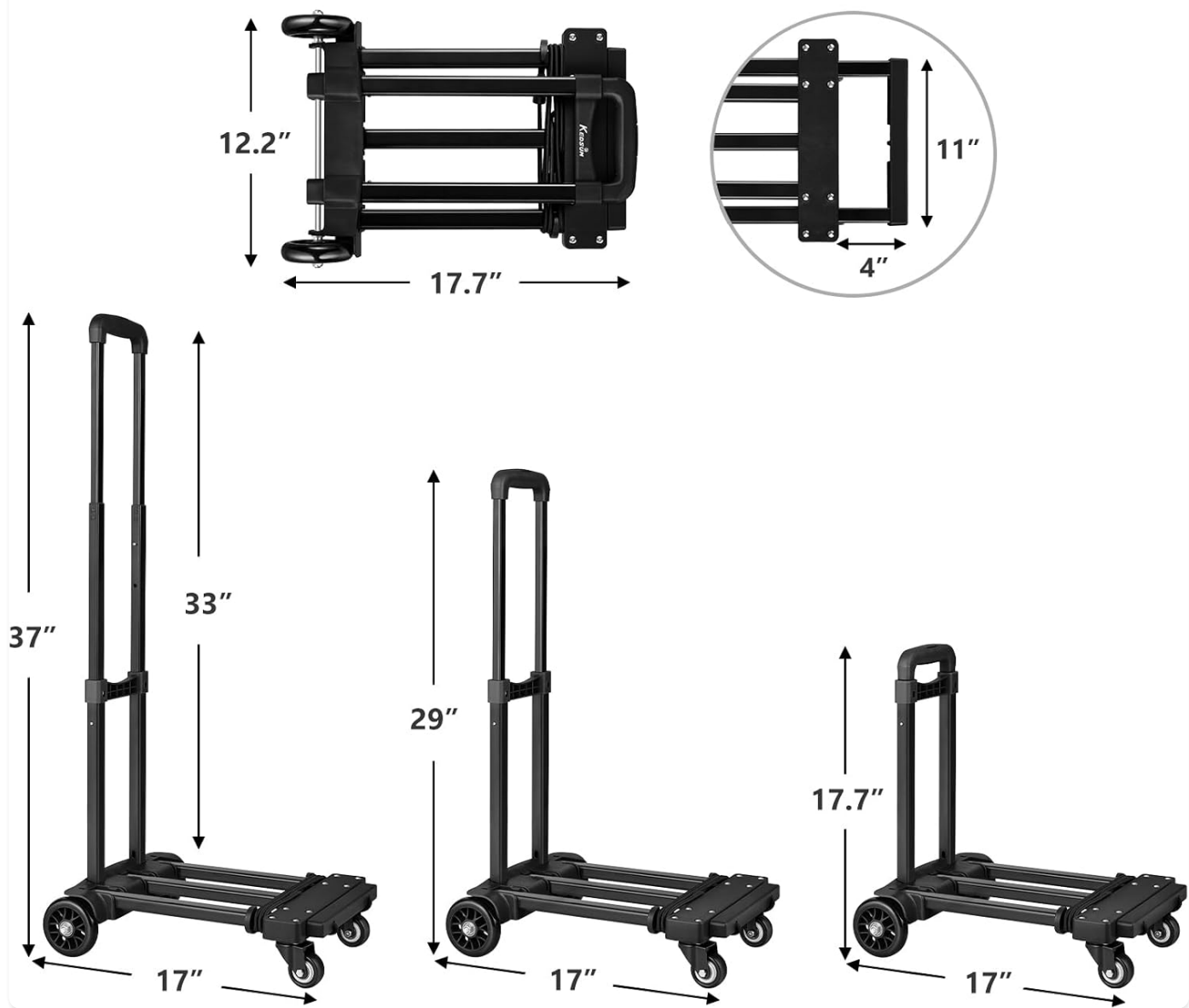
Figure 6: Visual representation of the cart's compact size and various dimensions for storage and use.
