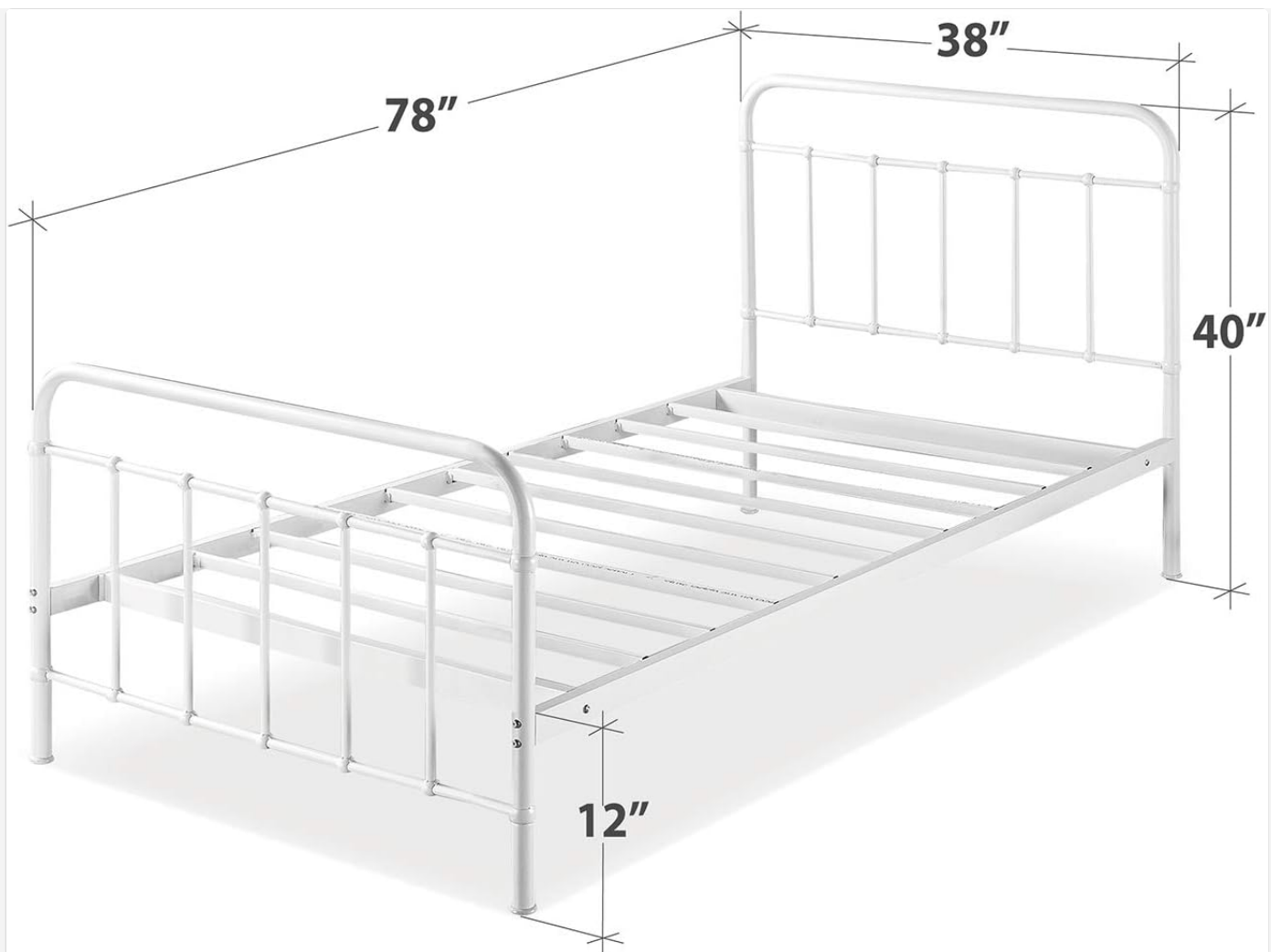
Image: Key dimensions of the Twin bed frame.
