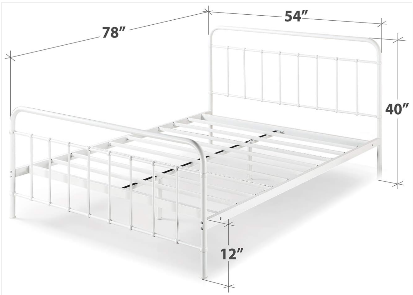
Image: A detailed diagram illustrating the key dimensions of the ZINUS Florence Full Panel Metal Platform Bed Frame.
