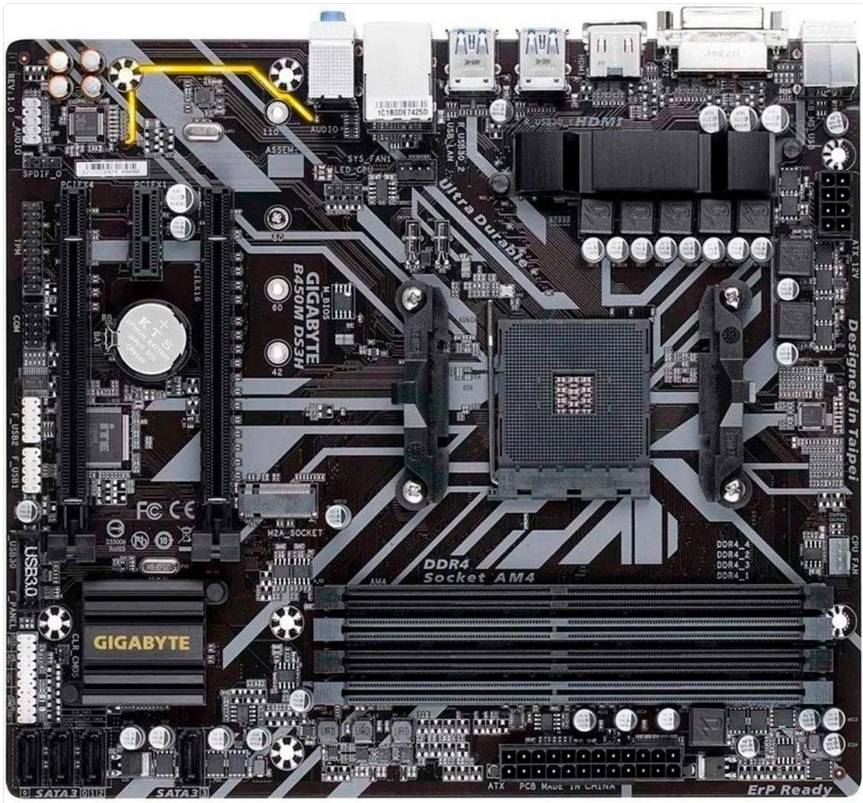
Image 2.3: Angled view of the motherboard, highlighting the M.2 slot and PCIe expansion slots.
