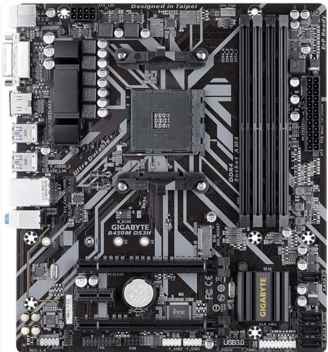
Image 2.1: Top-down view of the GIGABYTE B450M DS3H motherboard, highlighting key component locations.
