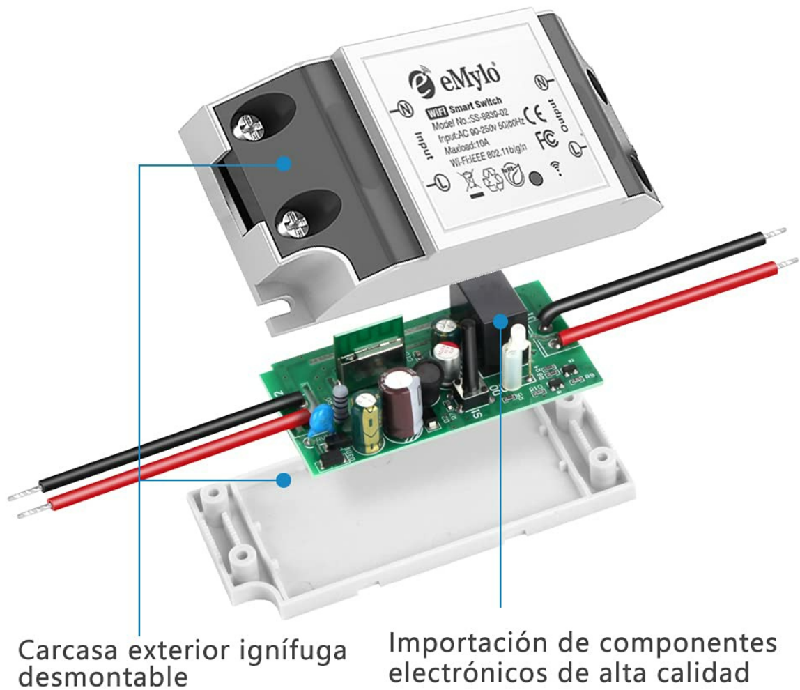
Image: Exploded view of the eMylo Smart WiFi Switch, illustrating its internal structure and connection points. The fire-retardant casing and high-quality electronic components are visible.
