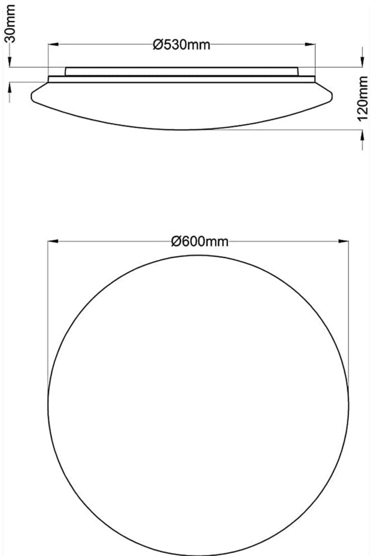
Image: Dimensional diagram of the ceiling light, showing a diameter of 600mm and a height of 120mm.
