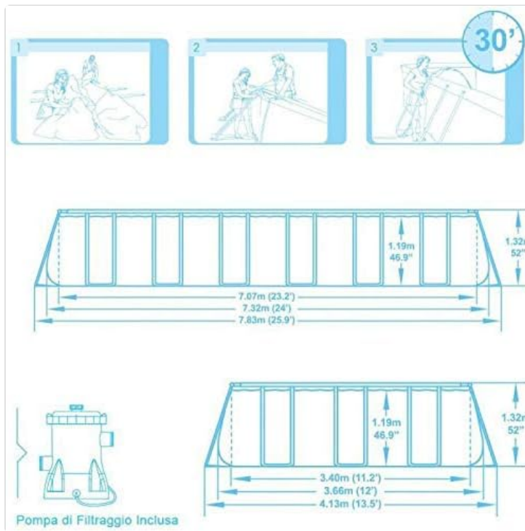
Image 4.1: An illustrative diagram showing the assembly steps and key dimensions of the Bestway Power Steel Rectangular Pool. It depicts the process of unfolding the liner, assembling the frame, and the overall dimensions of the pool (7.32m x 3.66m x 1.32m) and the filter pump connection.
