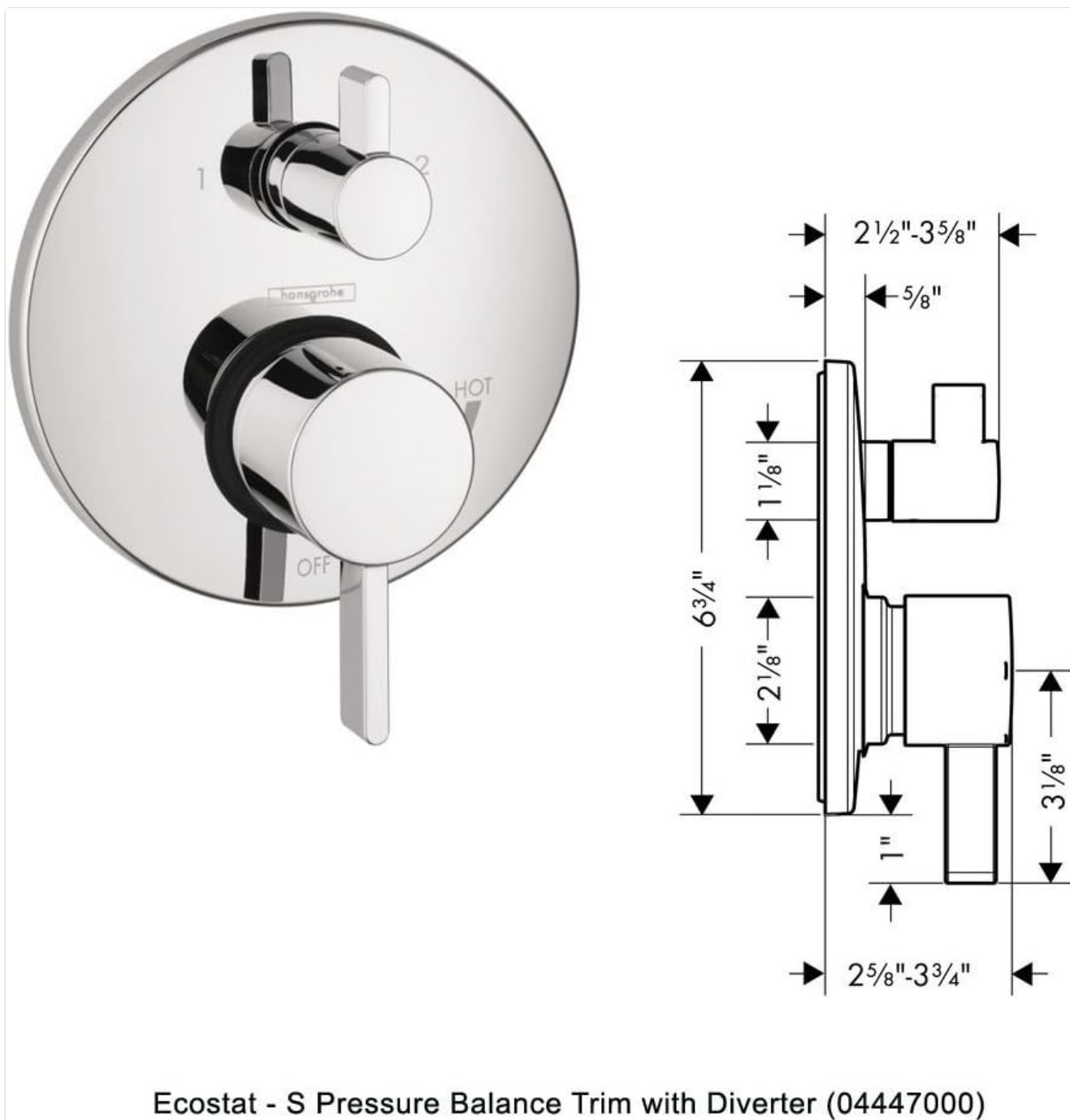
Figure 3: Dimensions for the Ecostat - S Pressure Balance Trim with Diverter (04447000). This diagram provides critical measurements for proper trim installation over the iBox.
