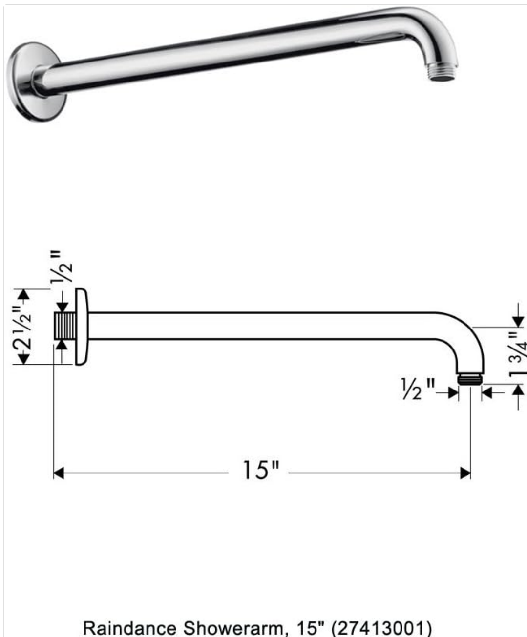
Figure 4: Dimensions for the Raindance Showerarm, 15 inches (27413001). This image shows the length and connection details for the shower arm.
