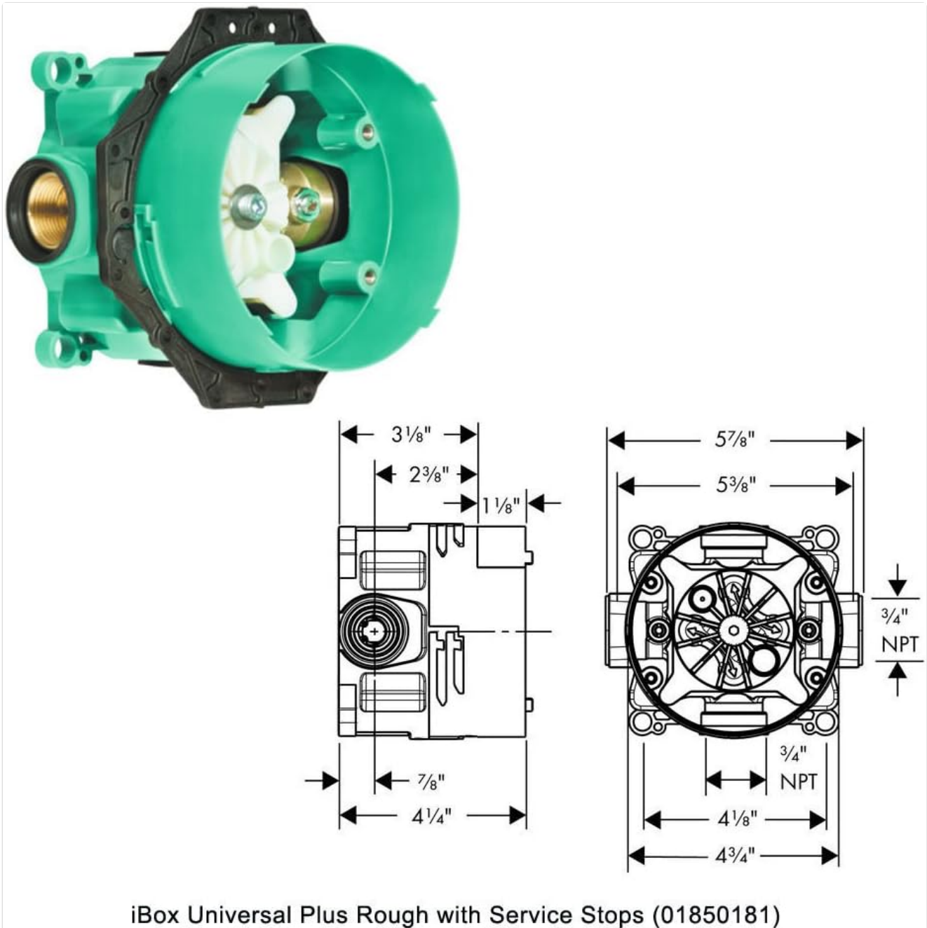
Figure 2: Detailed view and dimensions of the iBox Universal Plus Rough with Service Stops (01850181). This component is essential for the concealed installation of the shower valve.
