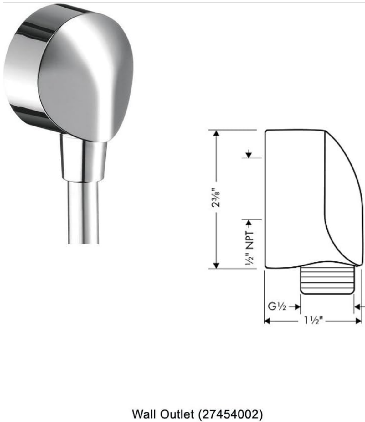
Figure 6: Dimensions for the Wall Outlet (27454002). This component provides the connection point for the handheld shower hose.
