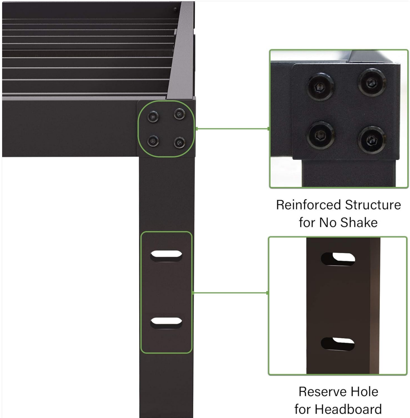
Figure 3.1: Detail of the reinforced structure at the corners and the pre-drilled holes for headboard attachment.
