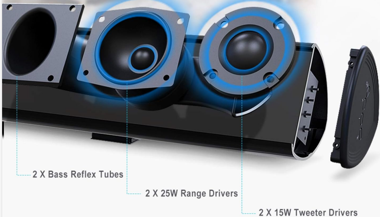
Image: An exploded view of the soundbar's internal components, highlighting two bass reflex tubes, two 25W range drivers, and two 15W tweeter drivers.
