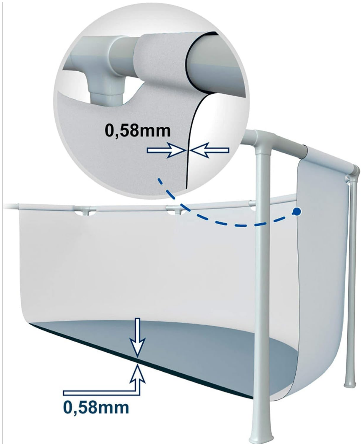
Image: Diagram illustrating the multi-layered construction and thickness of the pool wall (0.58mm), highlighting its durability.
