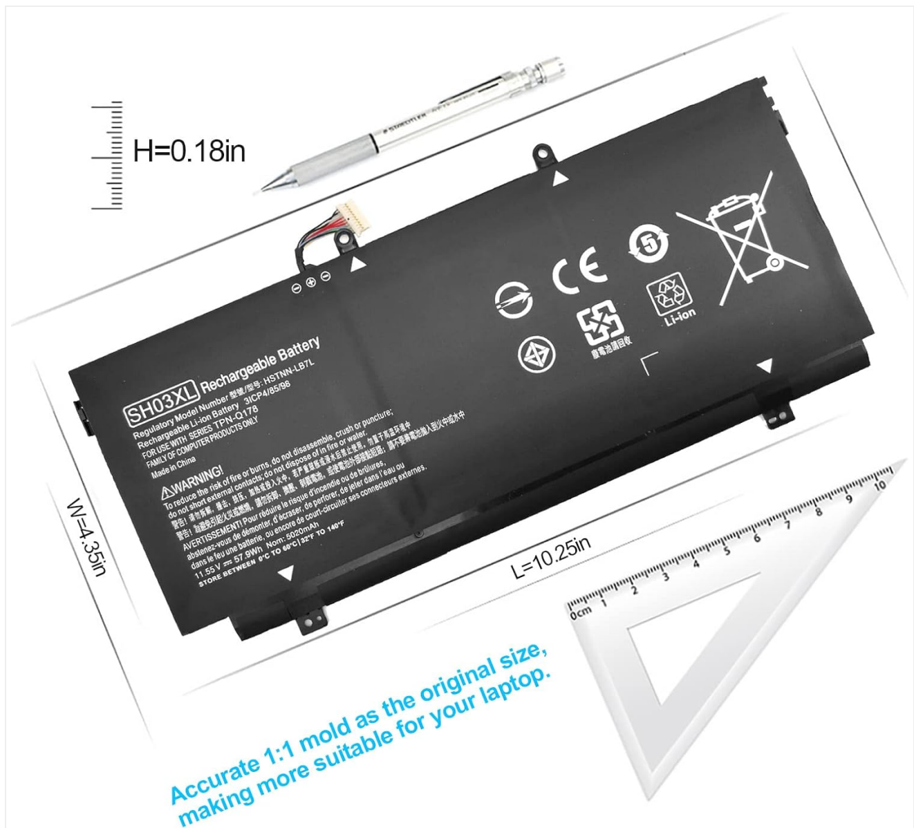
Image 2: Physical dimensions of the SH03XL battery, indicating it is an accurate 1:1 mold for the original size.
