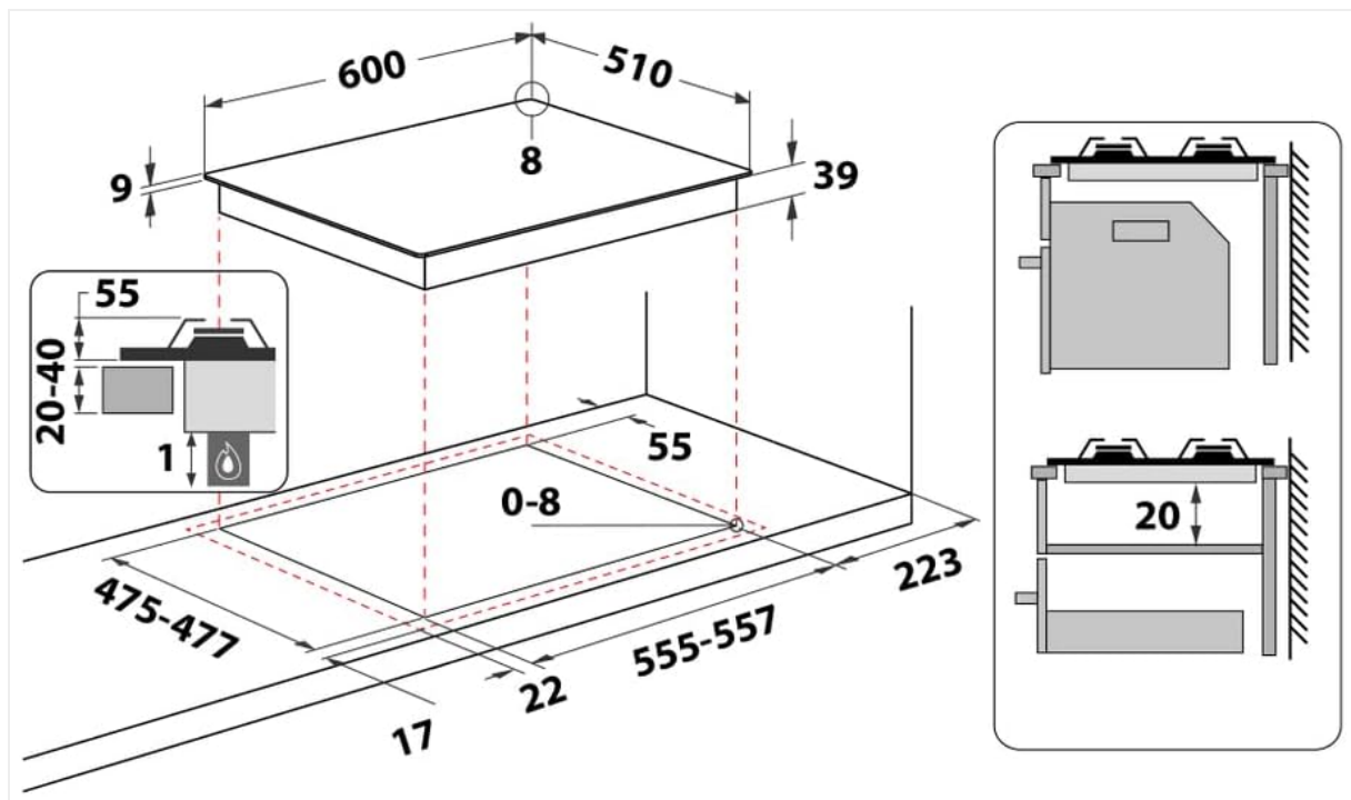
Image 2.1: Detailed installation diagram showing the hob's dimensions and required countertop cut-out measurements (e.g., 555-557mm width, 475-477mm depth).
