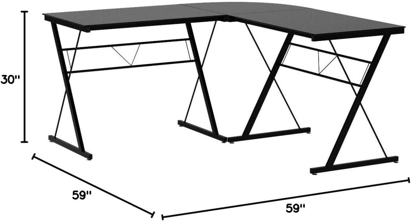
Image: Detailed dimensions of the L-shaped desk, indicating 59 inches for each side length and 30 inches in height.
