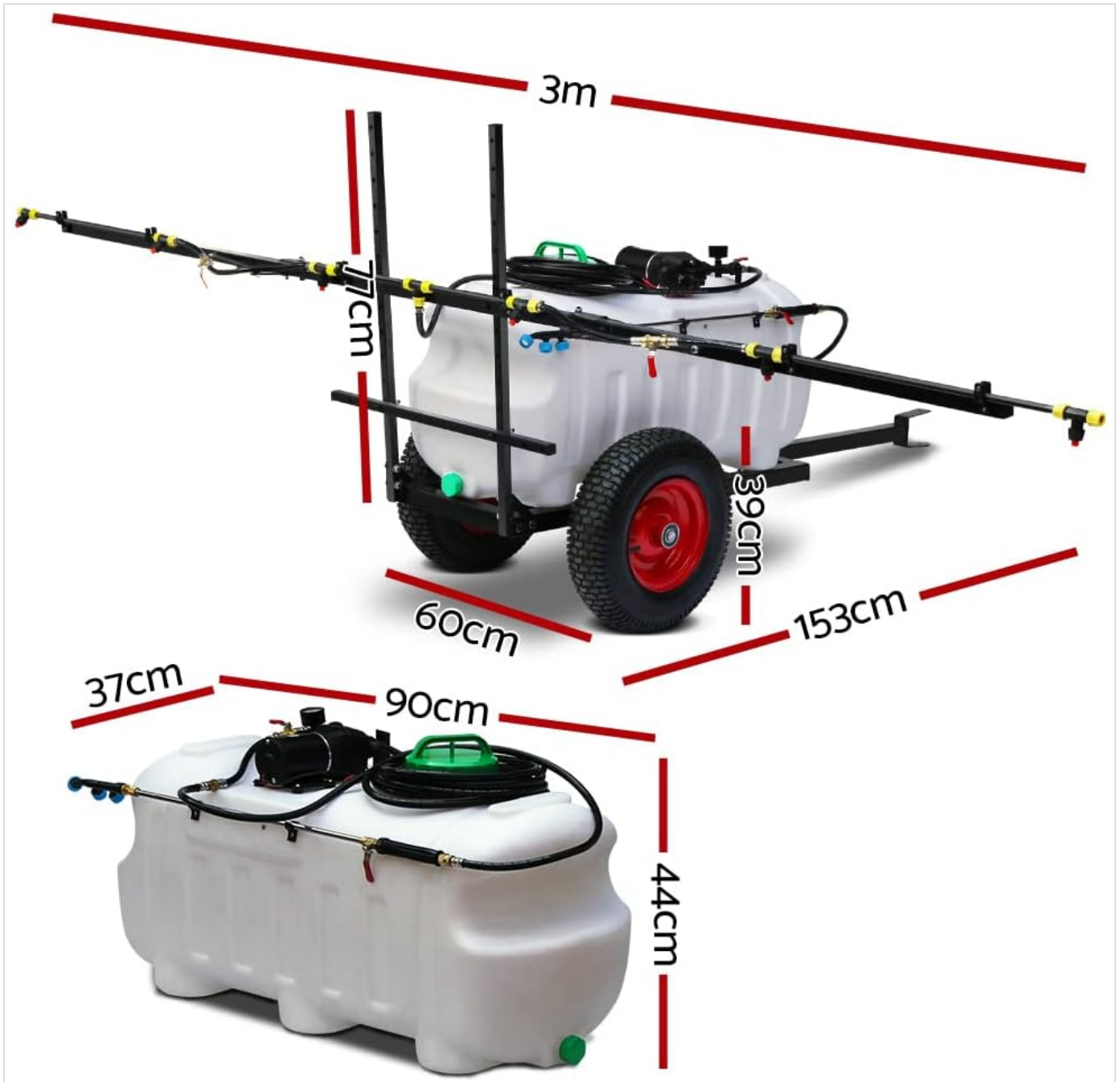
Figure 3: Key dimensions of the sprayer and tank for assembly and storage planning.
