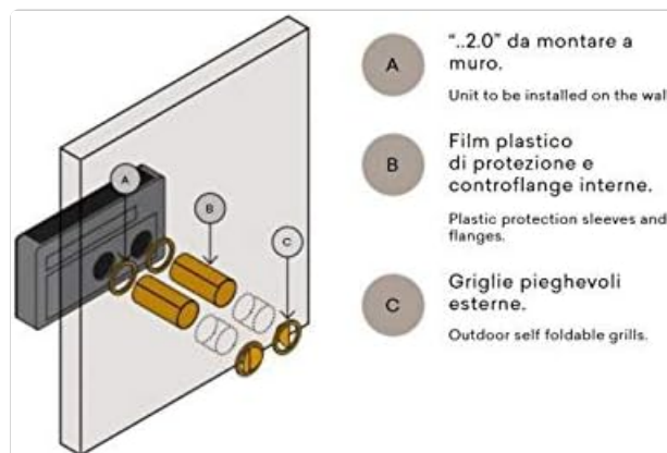
Figure 4.1: Diagram illustrating the key components and steps for wall installation, including the main unit (A), internal protection sleeves and flanges (B), and outdoor self-foldable grills (C).
