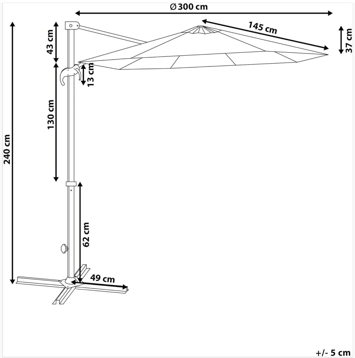
Image: Technical diagram illustrating the dimensions of the parasol, including height, width, and canopy diameter.
