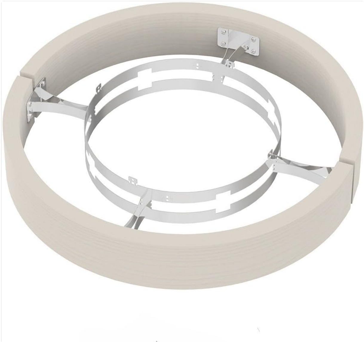
Figure 1: All components of the SAWO ARI-GUARD-W3-A Aspen Wooden Safety Rail, including the two wooden segments and the stainless steel frame.
