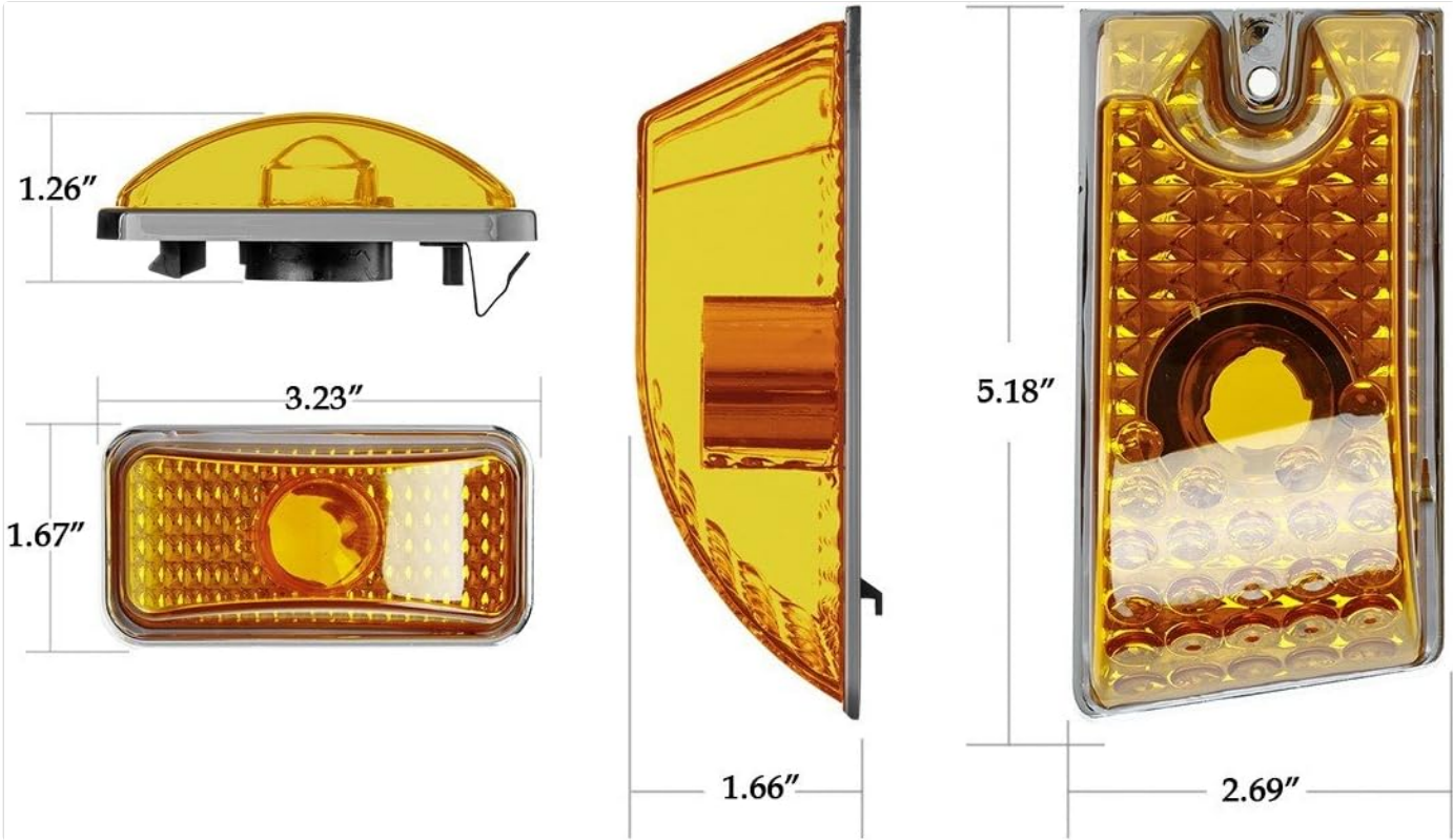
Image 6.1: Detailed dimensions of the Partsam Cab Marker Light for reference.
