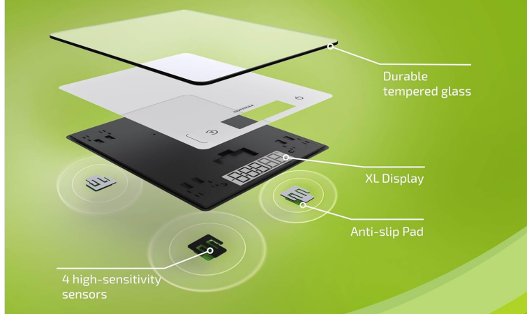
Image 4.1: Exploded view illustrating the internal components of the scale. This image highlights the durable tempered glass surface, the XL display, anti-slip pads, and the four high-sensitivity sensors that contribute to the scale's accuracy and quality.
