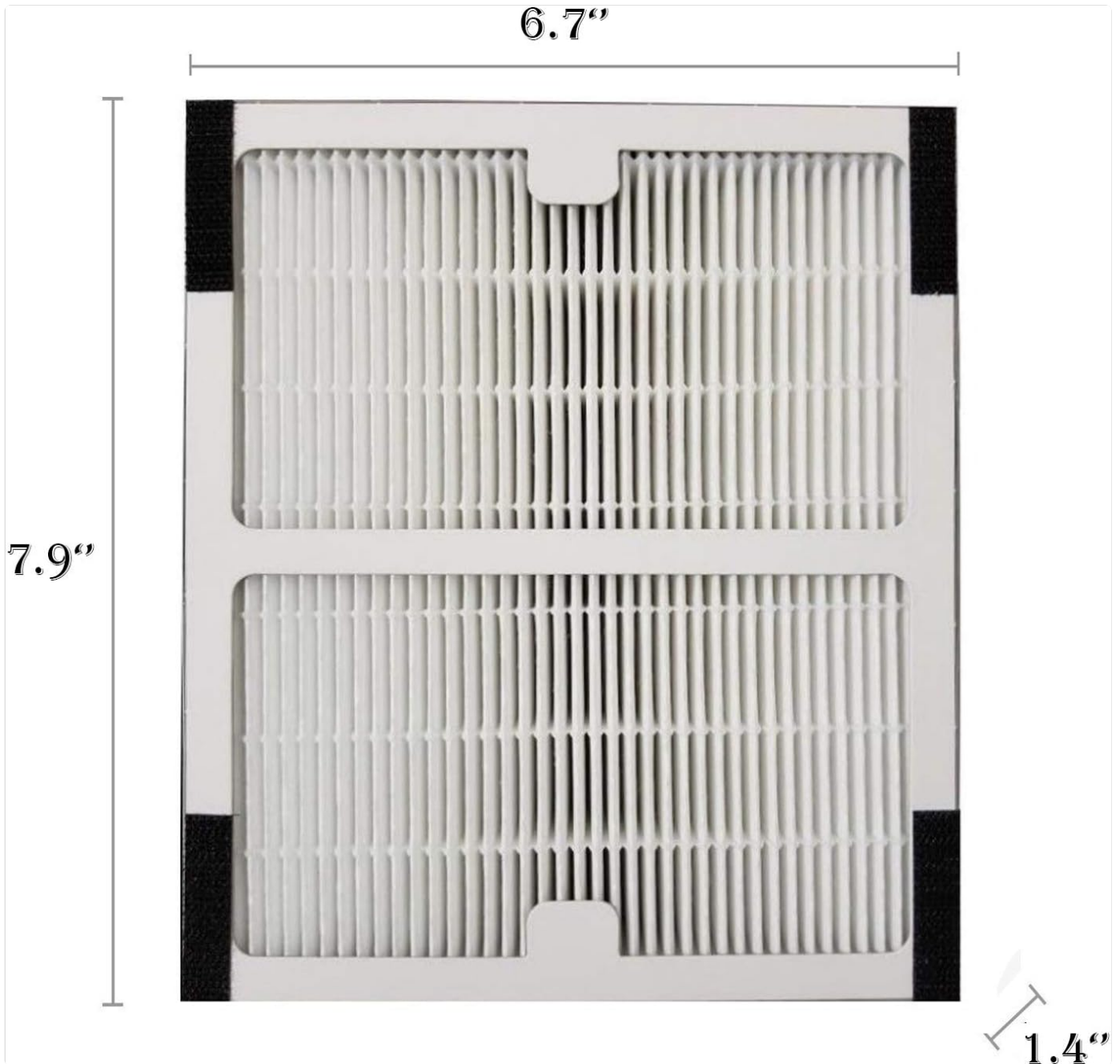
Image: Dimensions of the HEPA filter.
