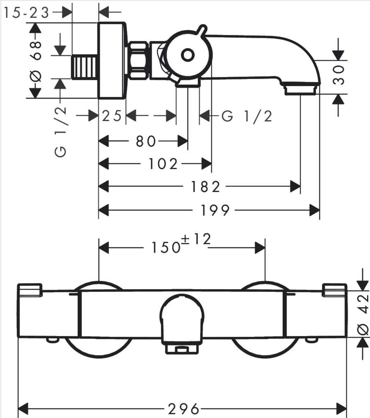
Figure 3: Detailed technical drawing providing dimensions for installation and planning of the Hansgrohe MyFox 13154000 mixer tap.
