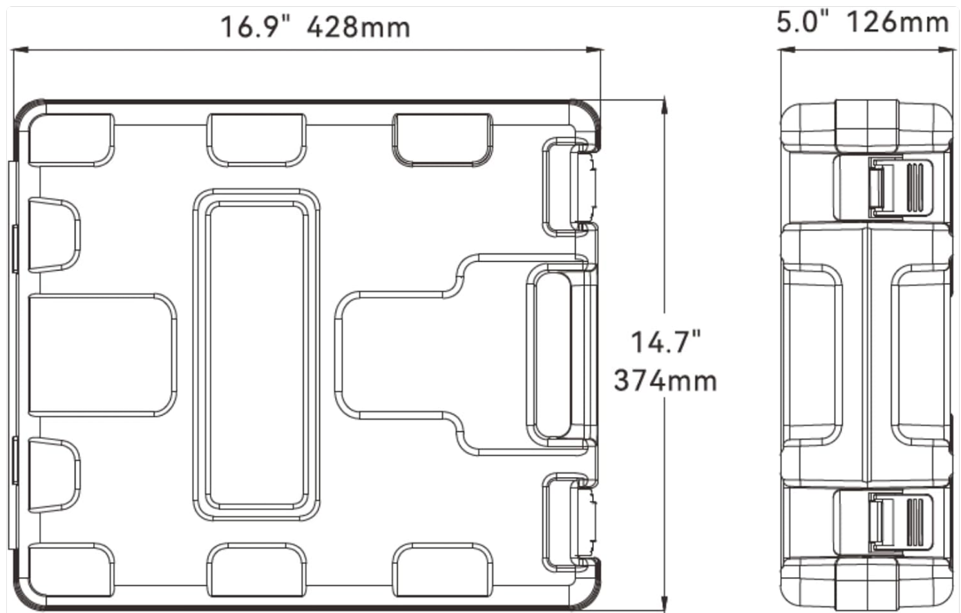
Figure 3.2: Dimensions of the portable carrying case.
