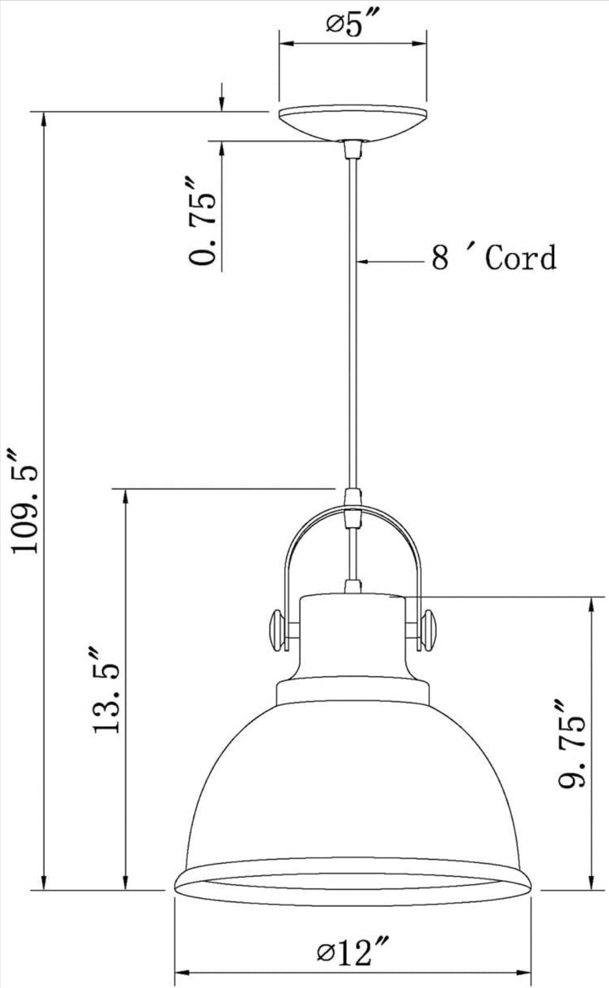
Figure 4.2.2: Technical drawing illustrating the dimensions of the Forte Lighting Harmon pendant. Key measurements include a 5-inch canopy diameter, 13.5-inch fixture height, 12-inch shade diameter, and an 8-foot cord.
