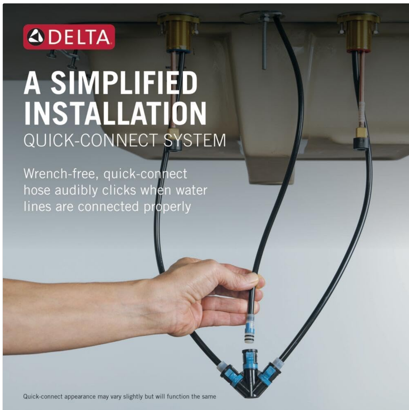
Image: A hand demonstrating the quick-connect system for the faucet's water lines, showing the audible click mechanism for secure installation.
