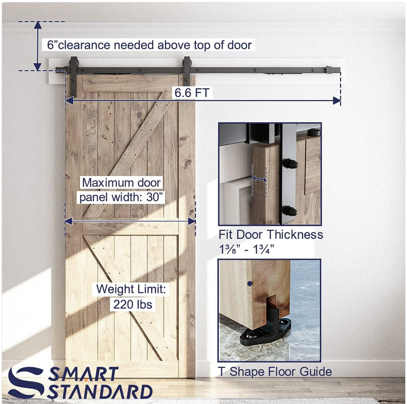
Figure 5: Key dimensions and floor guide installation details.
