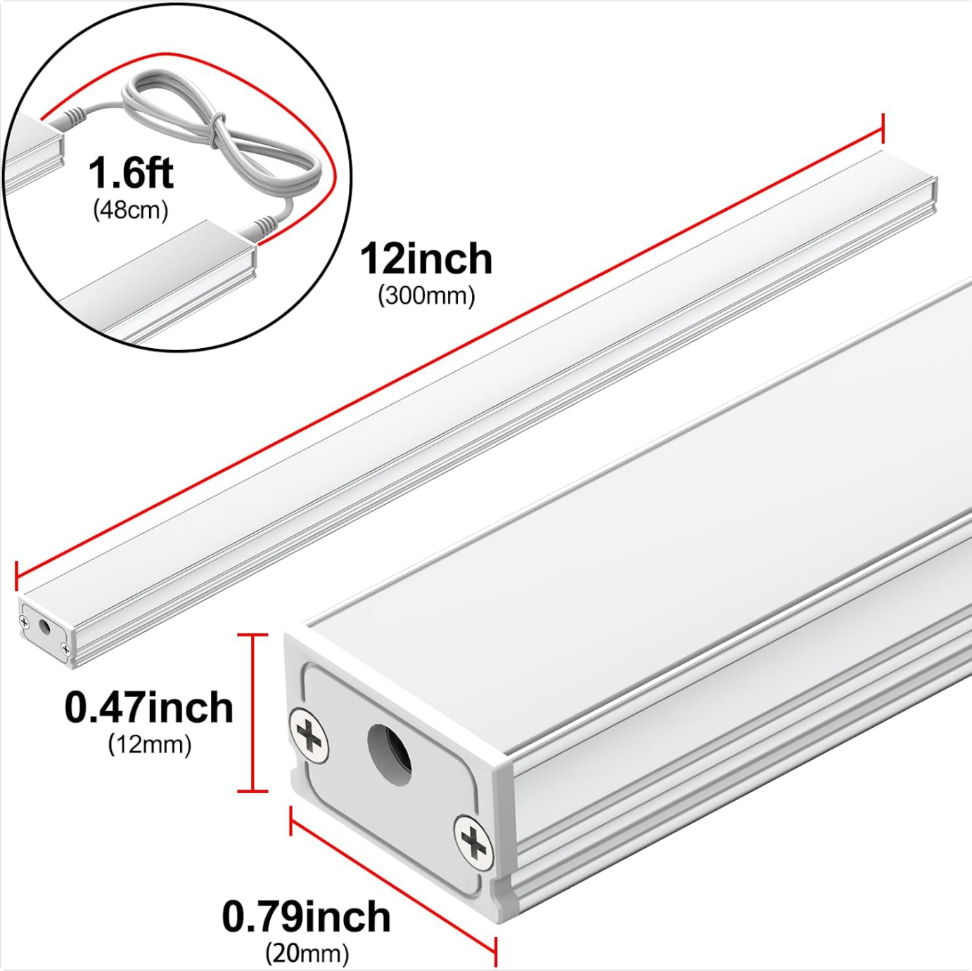
Figure 9: Detailed dimensions of the 12-inch LED light bar.
