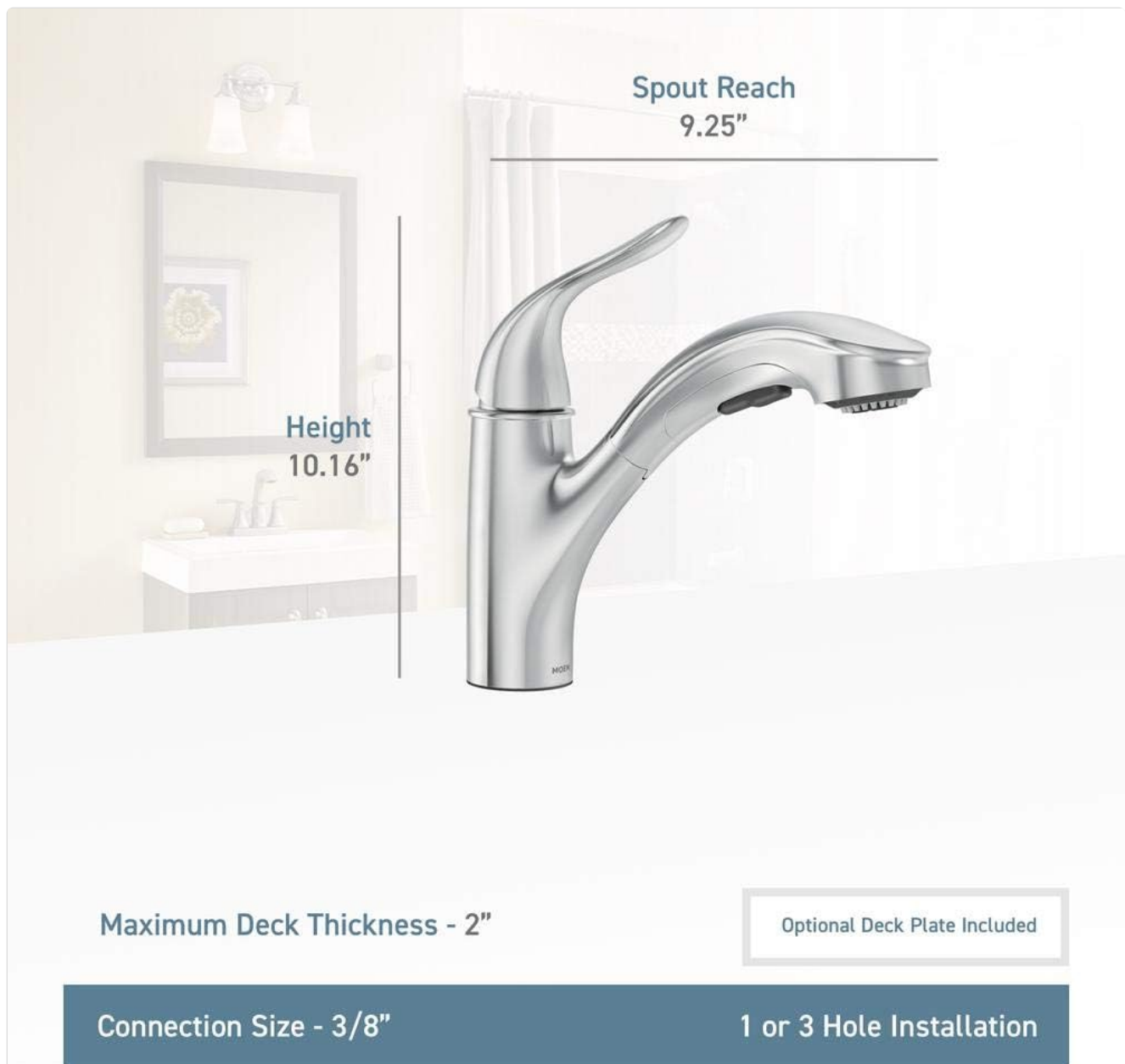
Figure 2: Faucet dimensions and installation details, including spout reach of 9.25 inches and height of 10.16 inches.
