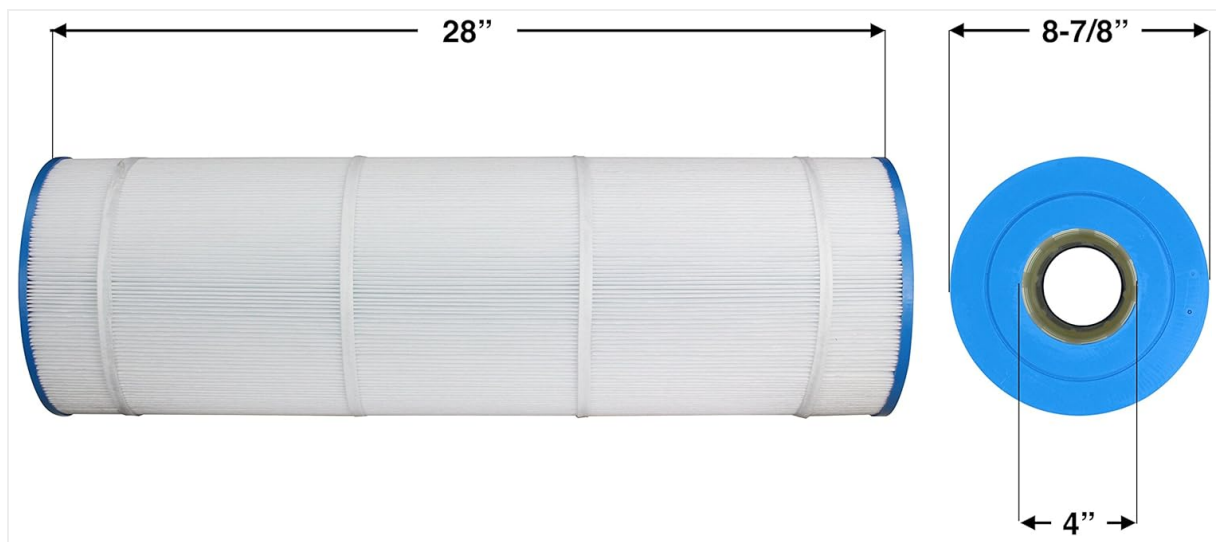
Image 3: Detailed dimensions of the filter cartridge, including length, outer diameter, and opening sizes.
