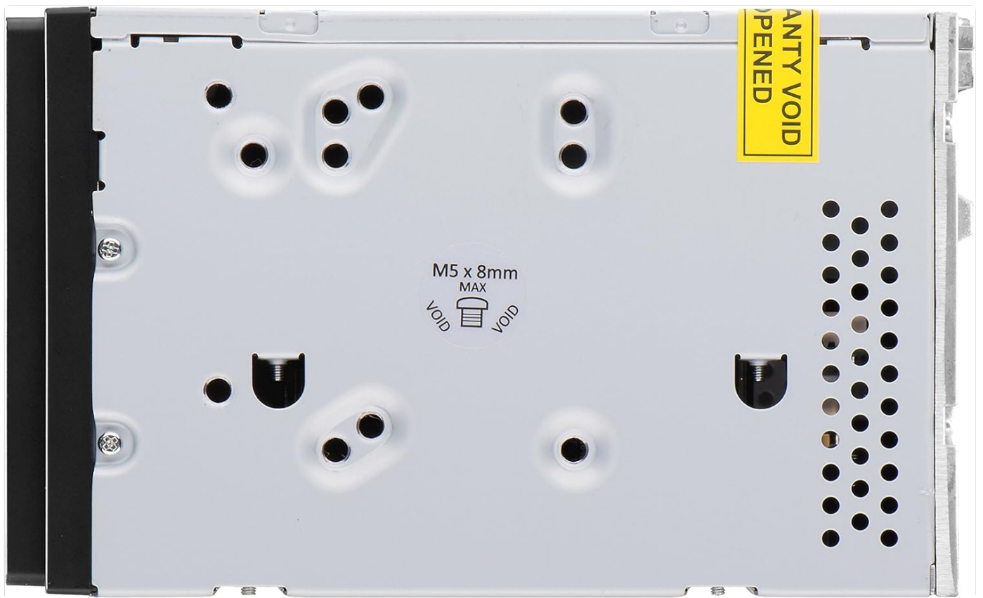
Figure 2: Rear view of the unit, illustrating mounting points.
