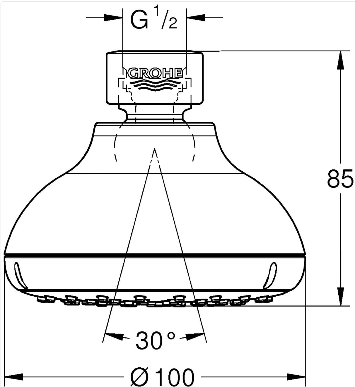
Diagram illustrating the dimensions and G 1/2 connection size of the GROHE Tempesta Classic 100 shower head, with a diameter of 100mm (approximately 4 inches).
