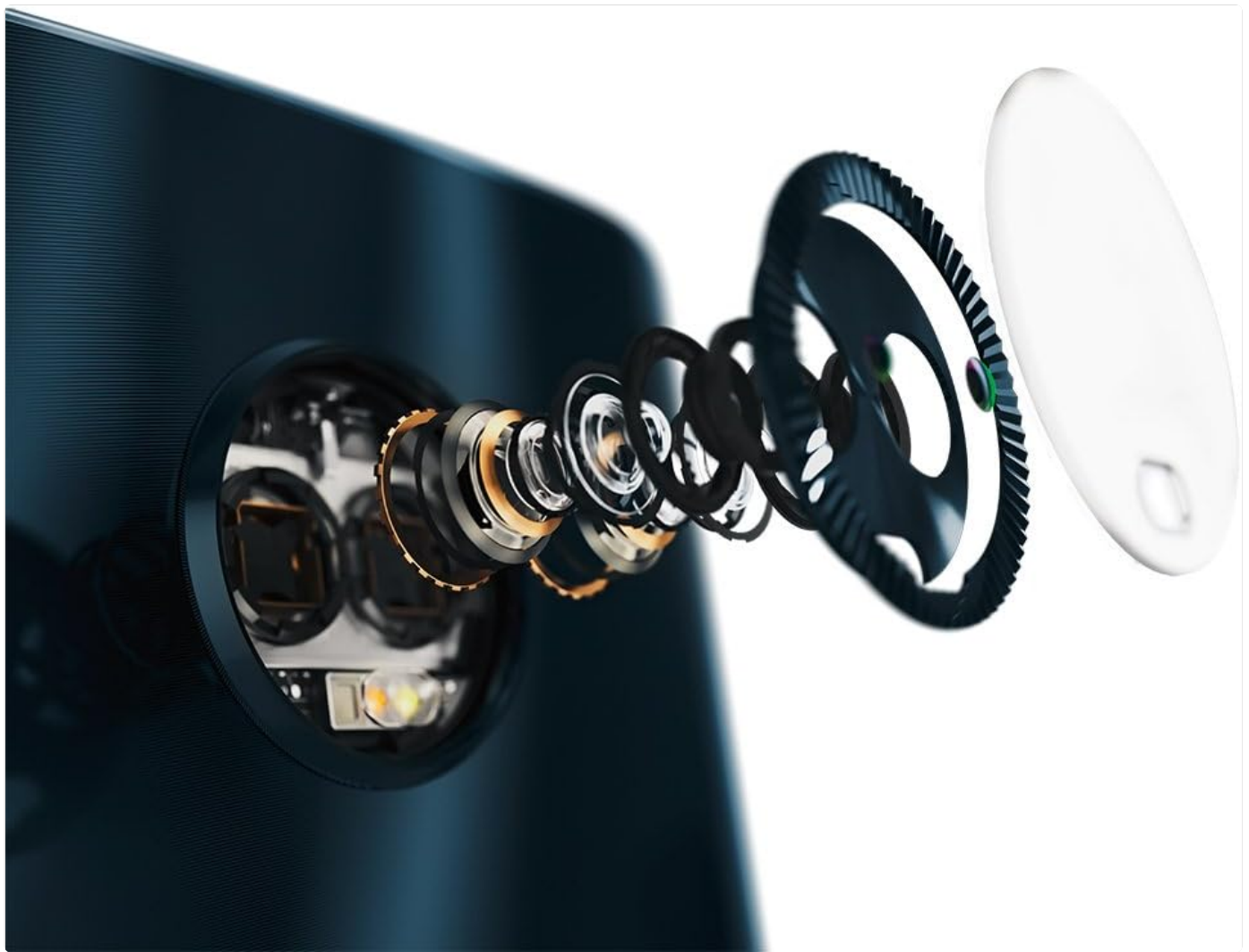
Figure 6: An exploded diagram illustrating the internal components of the Moto G6 Plus camera system.
