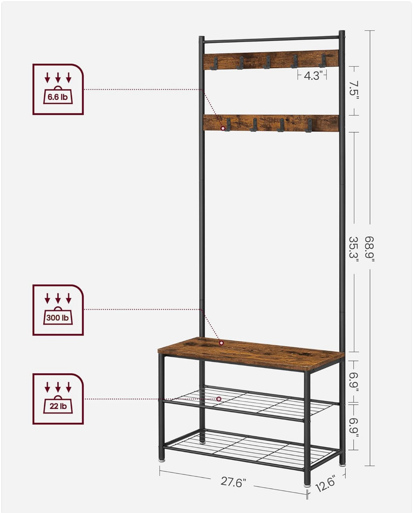
Image: Technical diagram illustrating the dimensions and maximum weight capacities for the hooks and bench.
