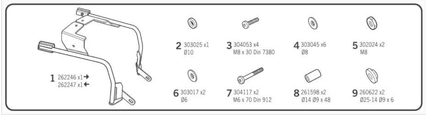
Image: Exploded view of the SHAD 3P System Fitting Kit components, showing various bolts, washers, spacers, and the main frame parts.
