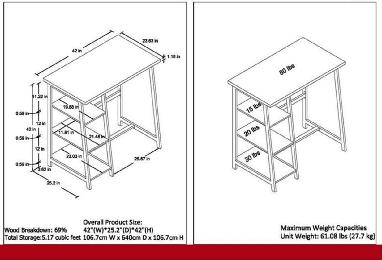
Image 3: Detailed diagram illustrating the dimensions and maximum weight capacities for the desk surface and shelves.
