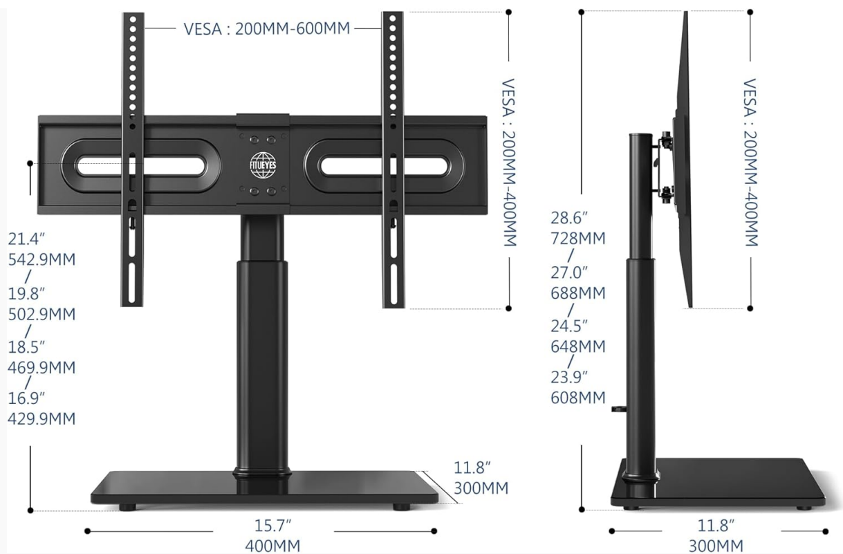
Figure 9.1: Dimensional specifications and VESA compatibility.
