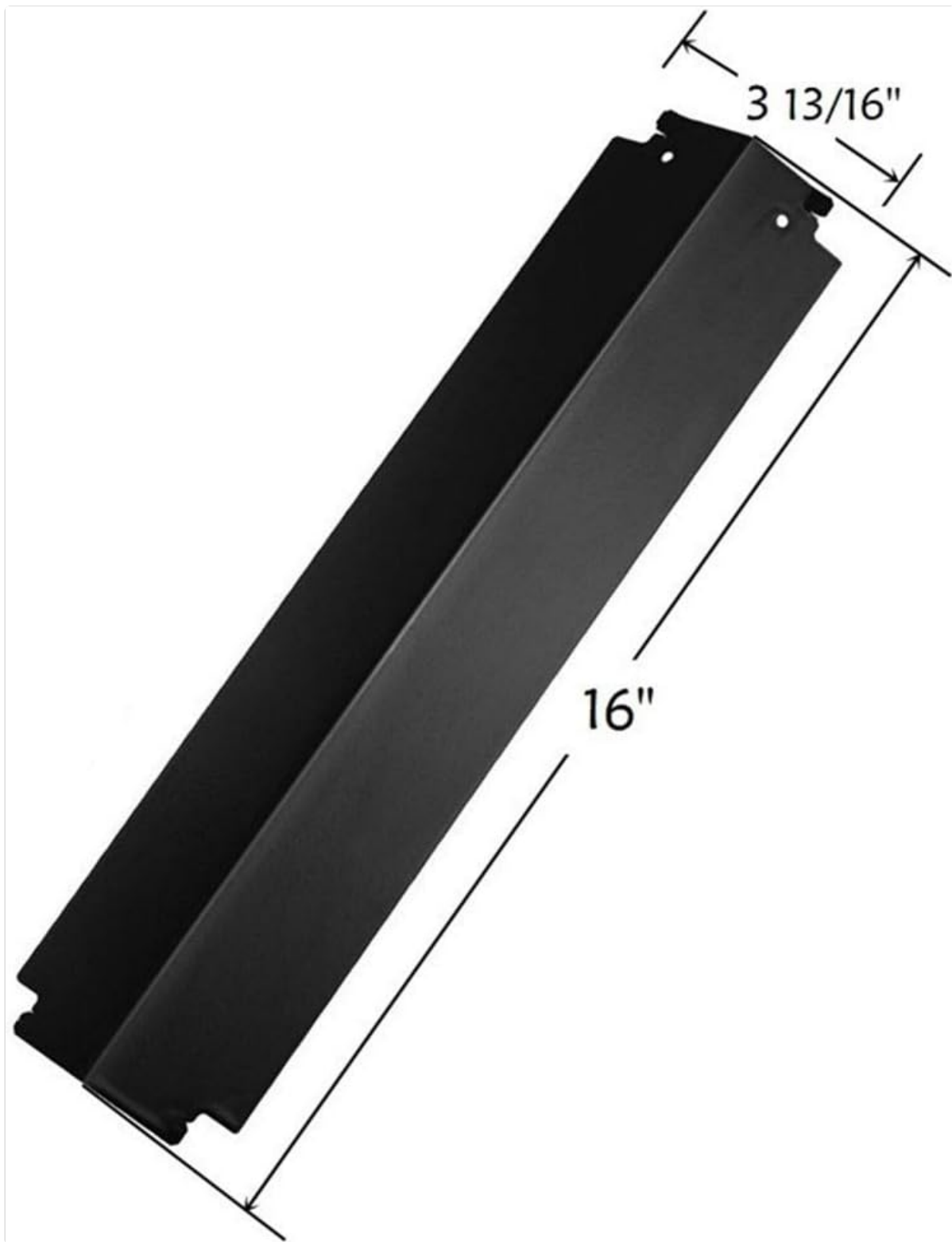
Image: Dimensions of the heat tent, crucial for ensuring compatibility.
