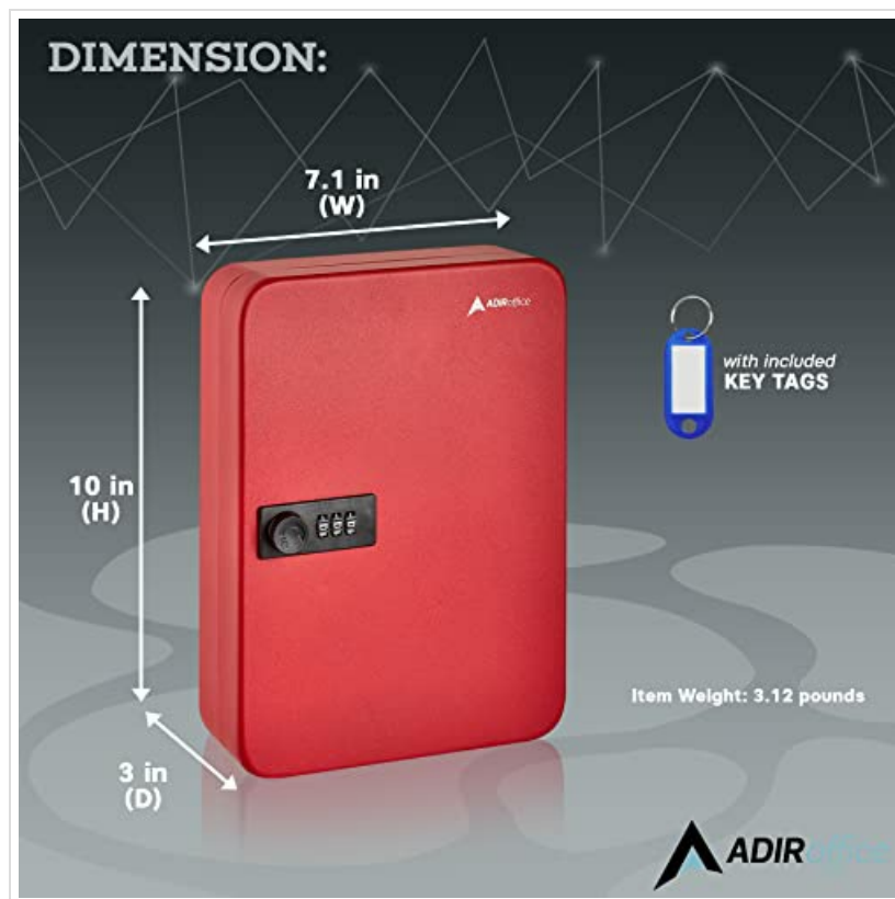
Figure 2: Cabinet dimensions for planning installation.
