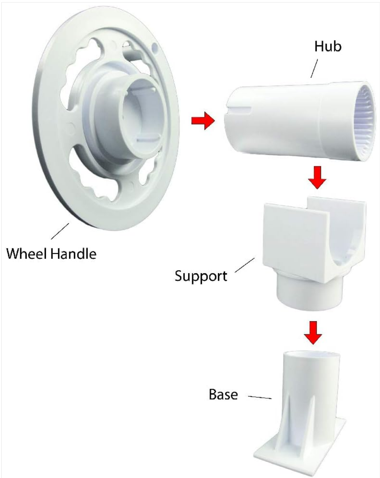
Figure 1: Exploded view of the solar cover reel components, showing the Wheel Handle, Hub, Support, and Base.
