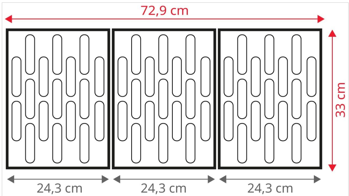
Image: Diagram detailing the dimensions of the three grill grates, each approximately 24.3 cm wide and 33 cm deep, combining for a total width of 72.9 cm.
