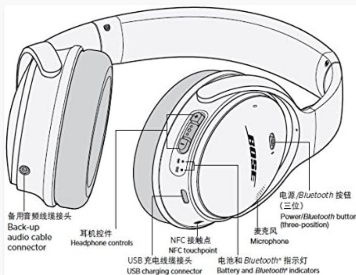
Figure 2: Detailed diagram of the right earcup, highlighting the Power/Bluetooth button, NFC touchpoint, USB charging connector, headphone controls, and microphone location.
