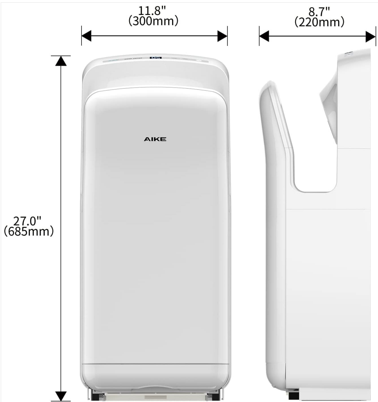
Image: Product dimensions for the AIKE AK2005H hand dryer, showing height, width, and depth.
