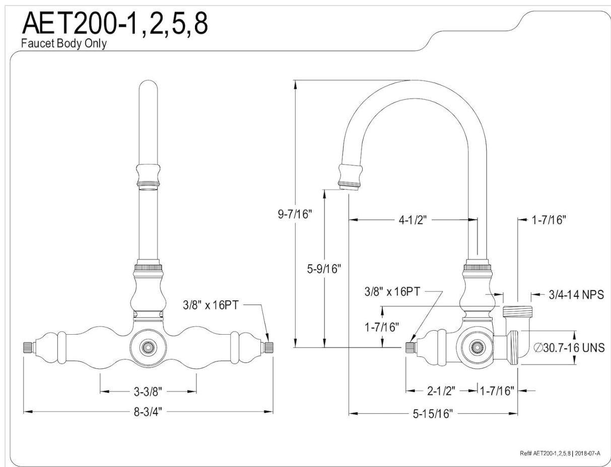
Figure 2: Detailed technical drawing of the AET200-1 faucet body, showing key dimensions including spout reach (4-1/2"), spout height (9-7/16"), and wall mount spacing (3-3/8").
